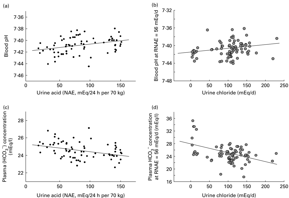
Fig. 1. (a) Blood pH at constant net acid excretion (NAE) rate ( r = 0.34 ; P < 0.005 ). (b) Blood pH at constant urinary chloride excretion rate (renal NAE (RNAE) = 56 mEq/d) ( r = 0.22 ; P < 0.05 ). (c) Plasma bicarbonate at constant NAE rate ( r = -0.36 ; P < 0.005 ). (d) Plasma bicarbonate at constant urinary chloride excretion rate (RNAE = 56 mEq/d) ( r = -0.45 ; P < 0.001 ). Adapted from Frassetto et al. (6) .
